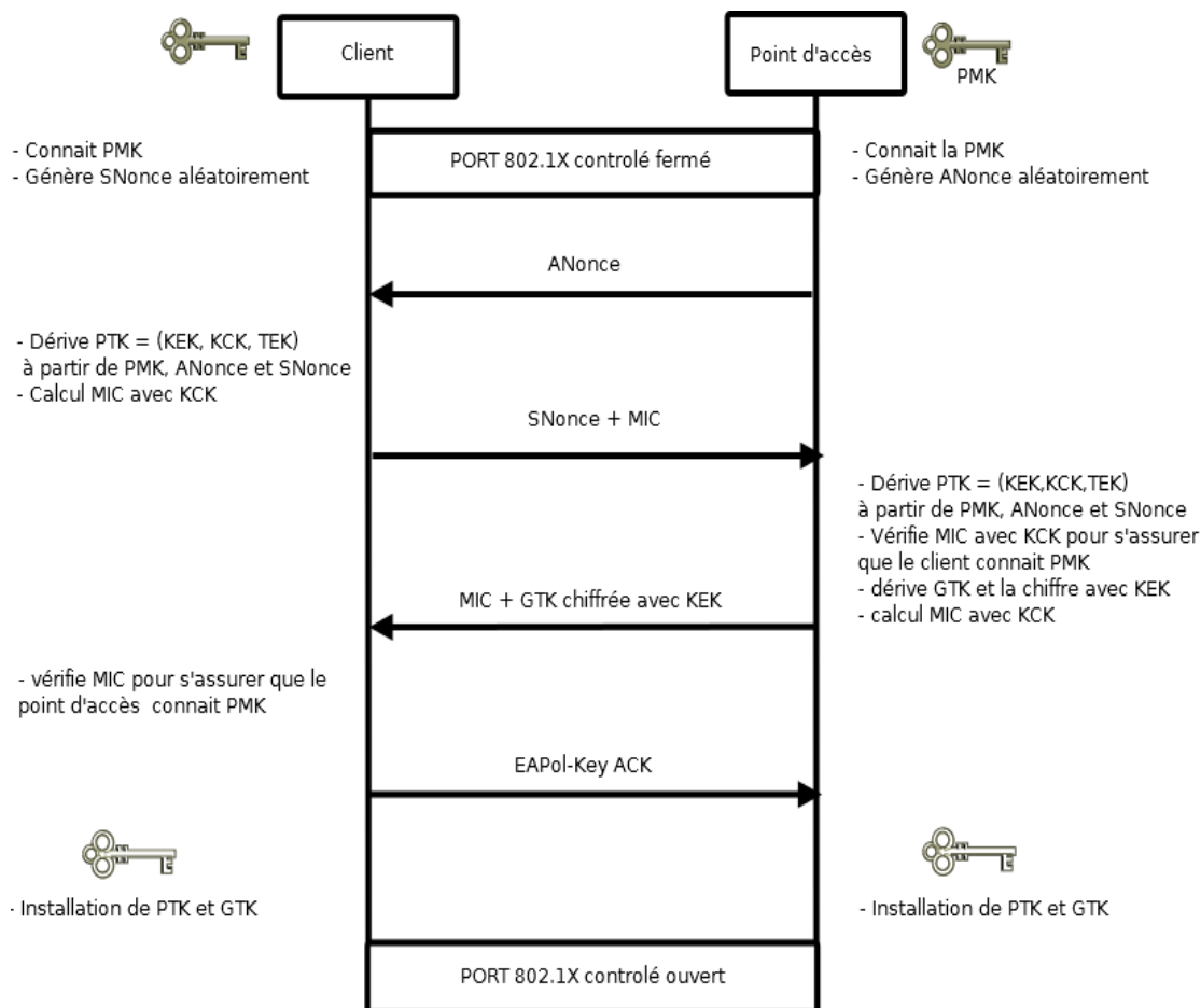
Figure 6 : 4 way handshake
