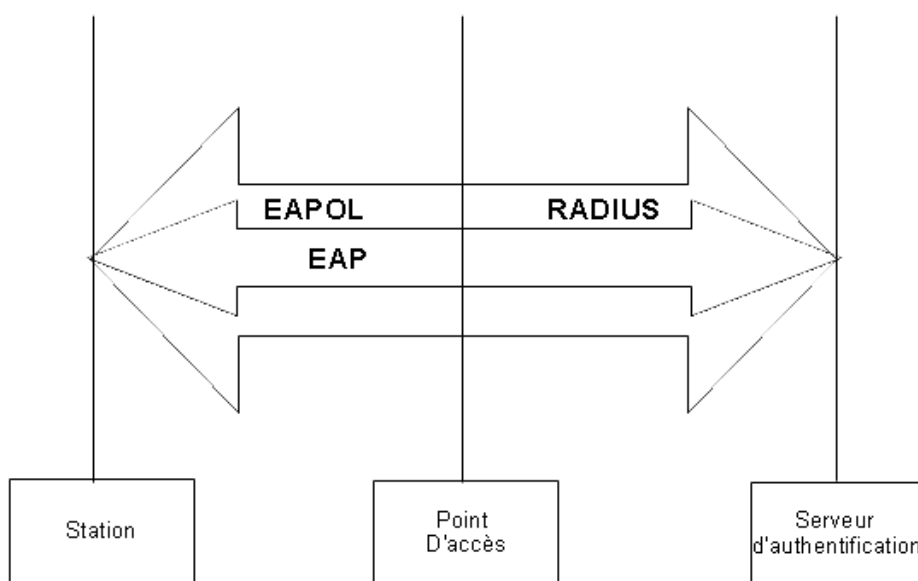
Figure 7 : Encapsulation EAP
