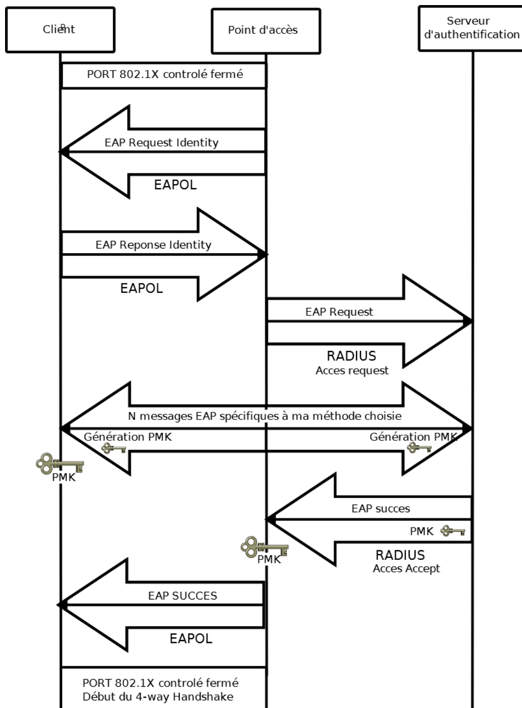
Figure 8 : Authentification 802.1X
